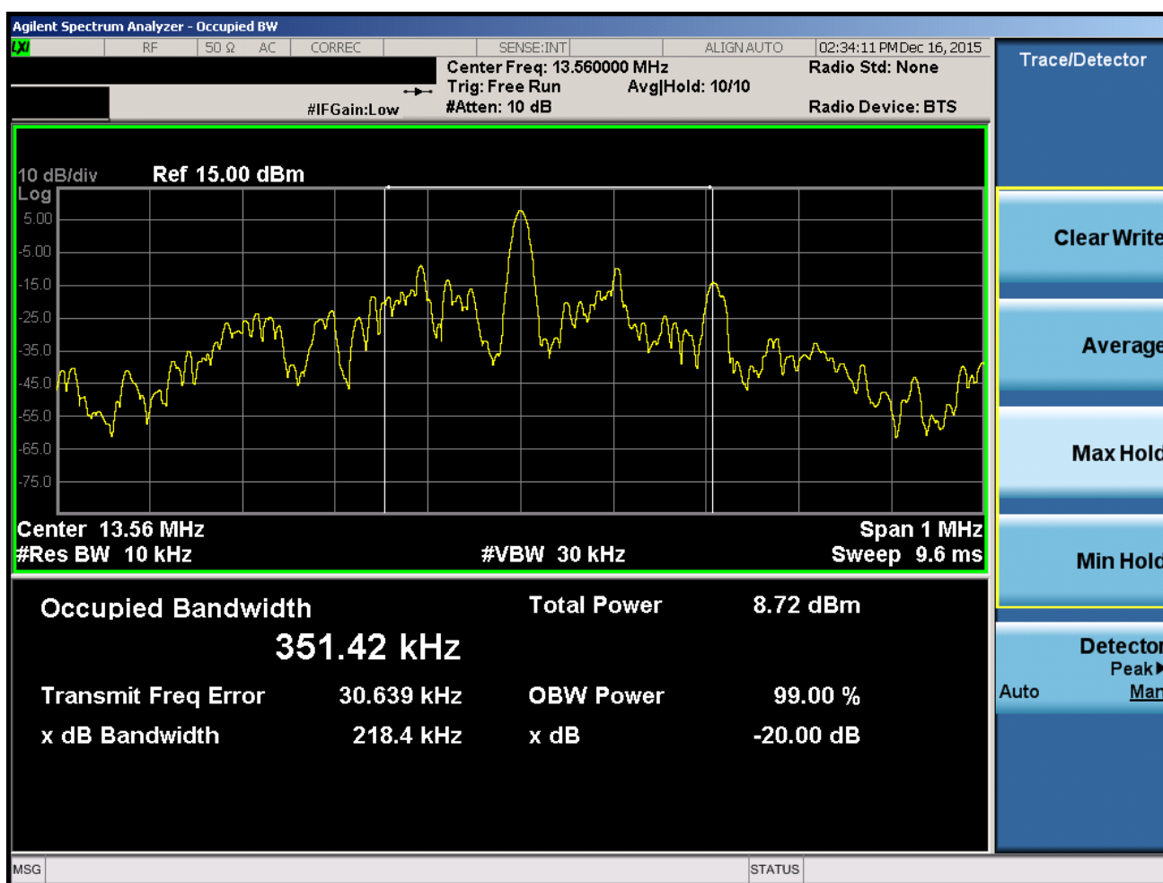
Figure 8-2. 20dB Bandwidth Plot
