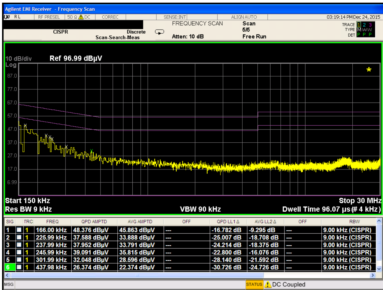
Plot 7-113. Line Conducted Plot with 802.11a UNII Band 2A (L1)
