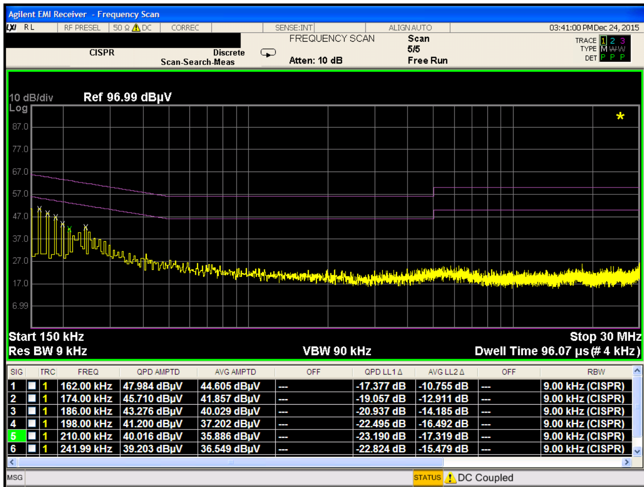
Plot 7-118. Line Conducted Plot with 802.11a UNII Band 3 (N)
