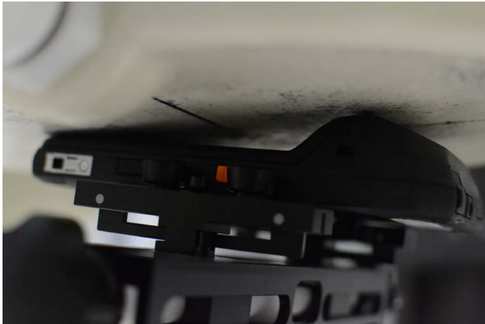
SAR Test Setup Photo 8: Back Side at 0.0 cm with Standard Battery
