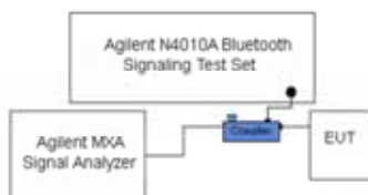
Figure 9-5 Bluetooth Power Measurement Setup
