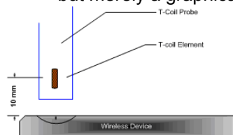
Figure 4-11 Measurement Distance
