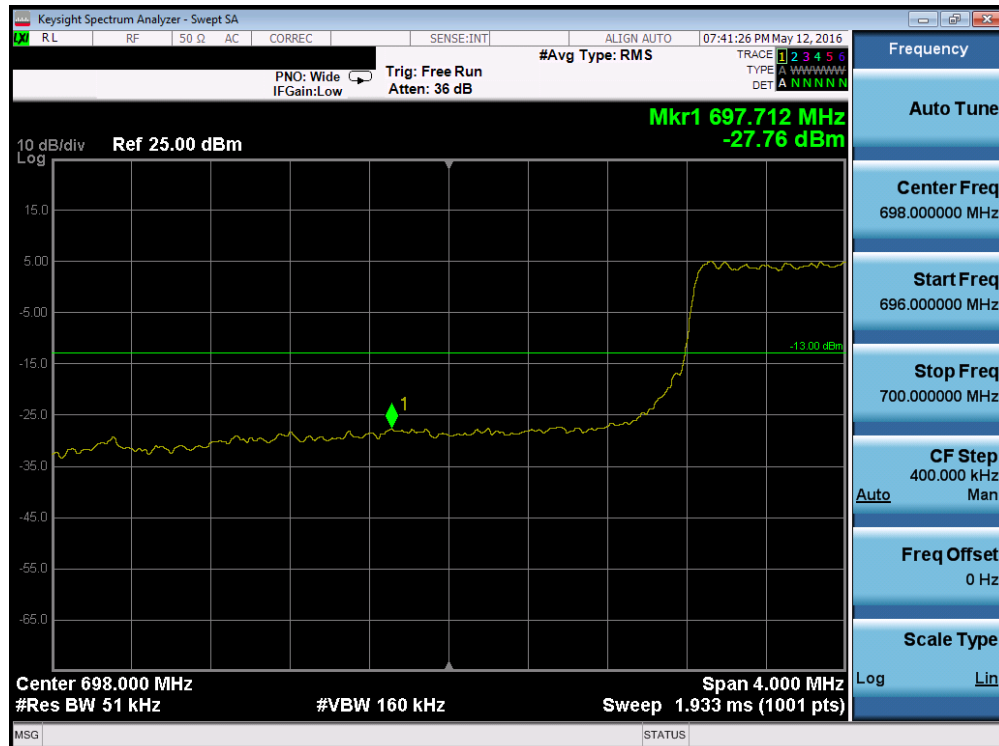
Plot 7-92. Lower Band Edge Plot (Band 12 – 5.0MHz QPSK – RB Size 25)
