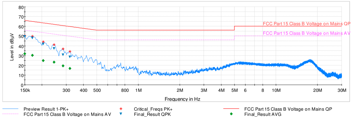
Plot 7-55. Line-Conducted Test Plot (N)
