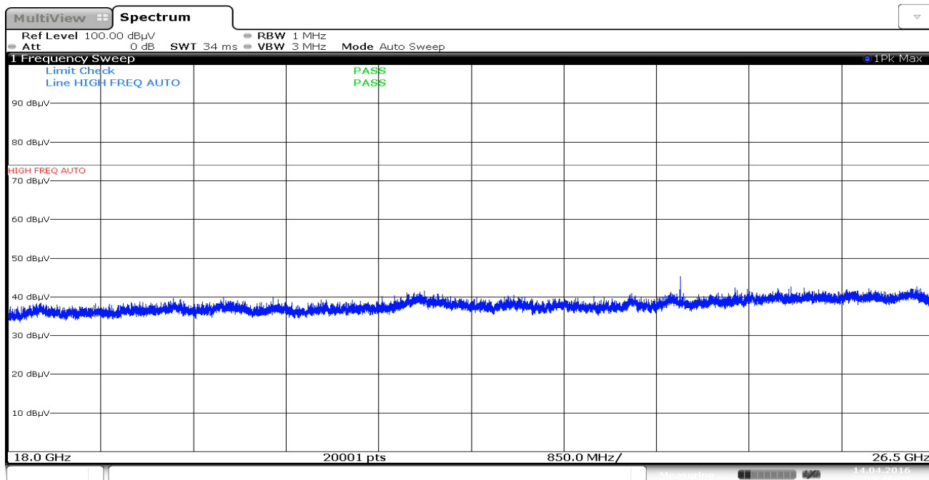
Plot 7-49. Radiated Spurious Plot above 18GHz (Pol. V)
