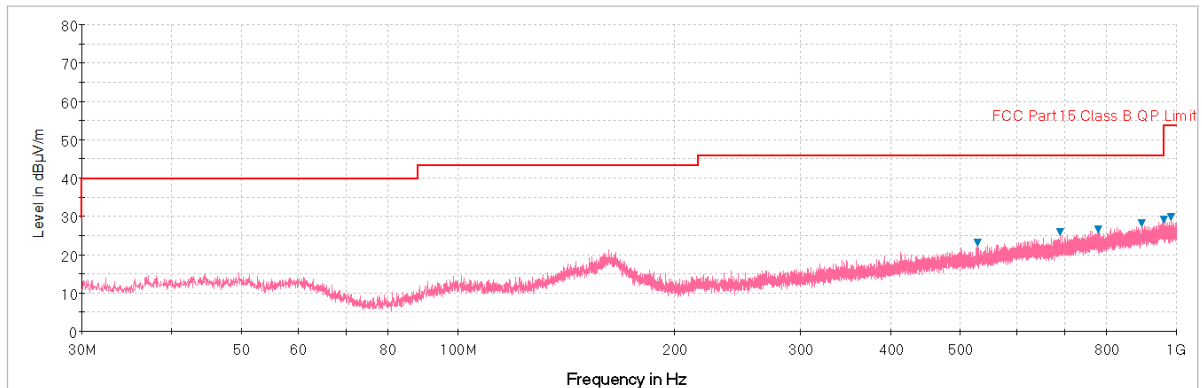
Plot 7-52. Radiated Spurious Plot below 1GHz (Pol. H)
