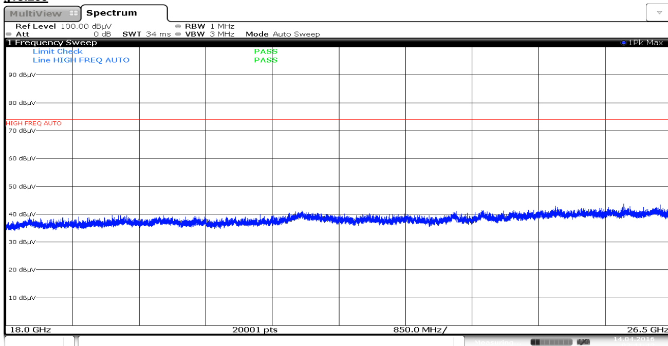
Plot 7-48. Radiated Spurious Plot above 18GHz (Pol. H)
