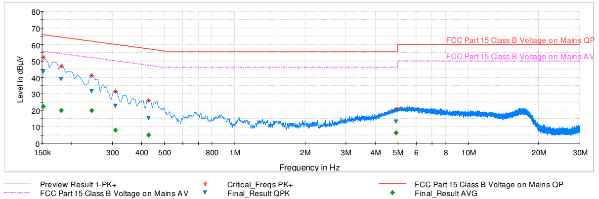
Plot 7-54. Line-Conducted Test Plot (L1)
