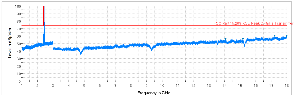
Plot 7-47. Radiated Spurious Plot above 1GHz (BT – Ch. 78, Ant. Pol. V)
