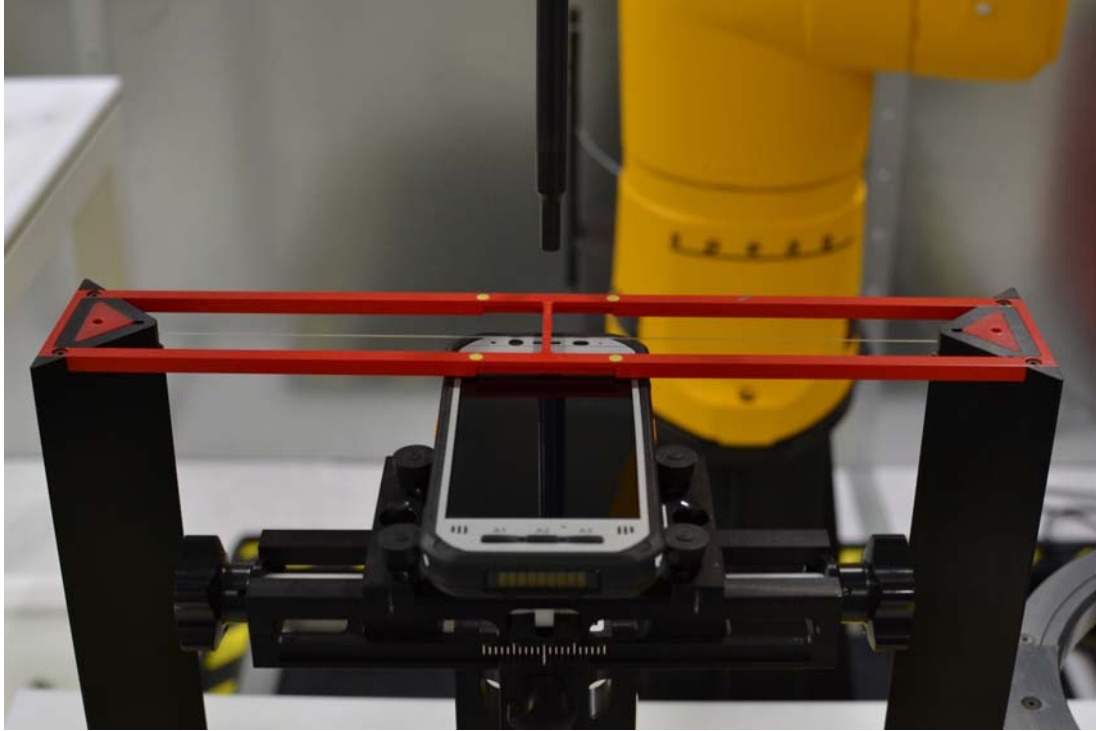
Figure 18-1 Ear Reference Point HAC Phantom Alignment (Standard Battery)
