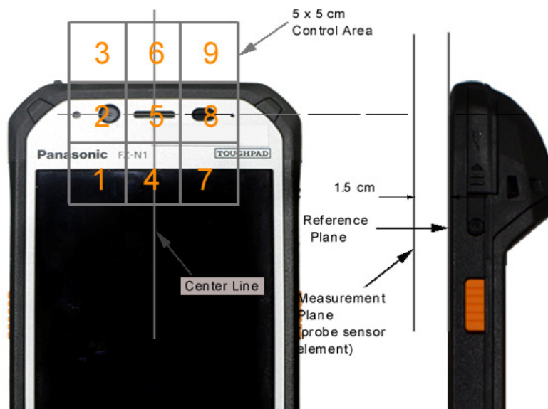
Figure 18-5 5x5 Scan grid above WD
