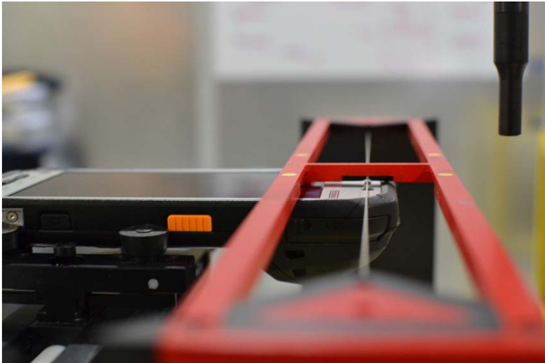
Figure 18-2 HAC Phantom Plane Alignment (Standard Battery)
