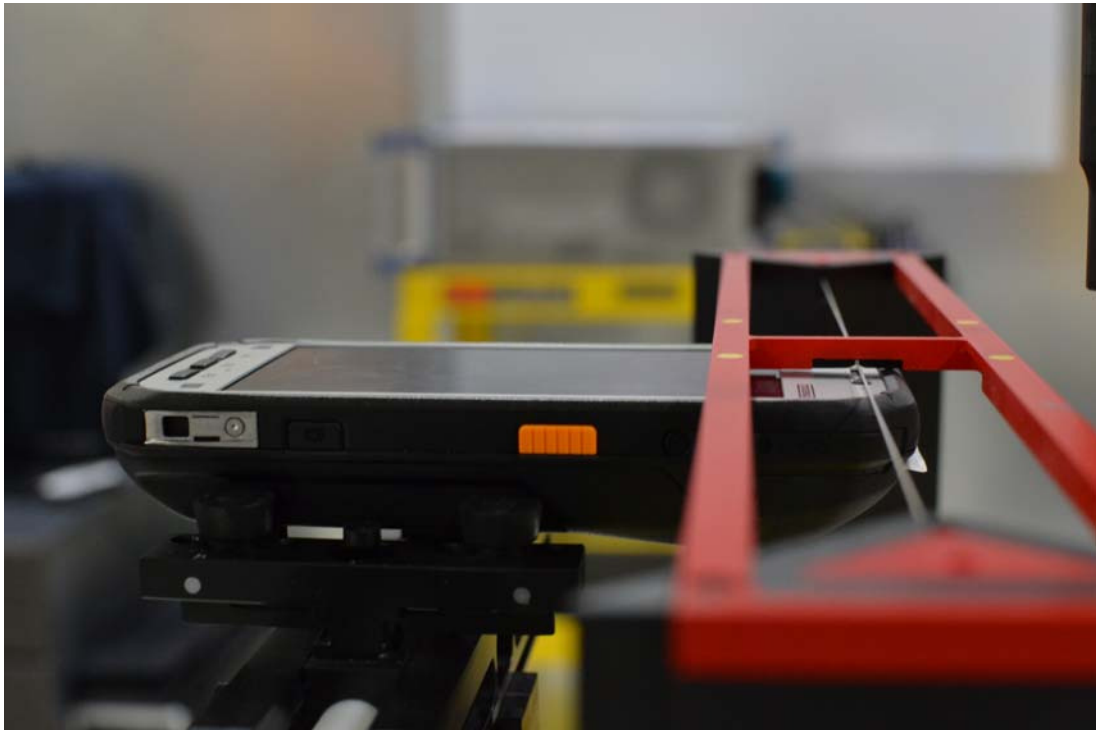
Figure 18-4 HAC Phantom Plane Alignment (L-Battery)
