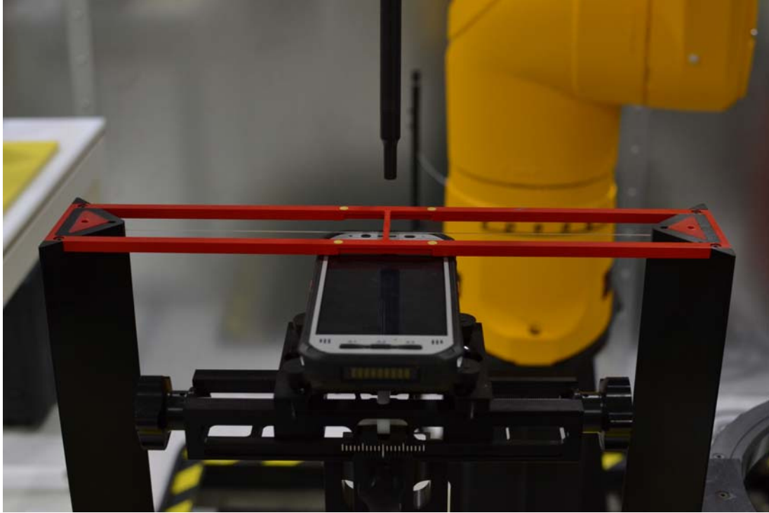
Figure 18-3 Ear Reference Point HAC Phantom Alignment (L-Battery)
