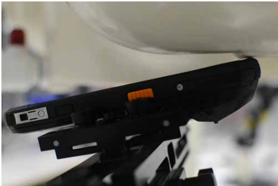
SAR Test Setup Photo 6 – Left Tilt with Standard Battery
