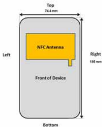
Figure F-2 NFC Antenna Locations
