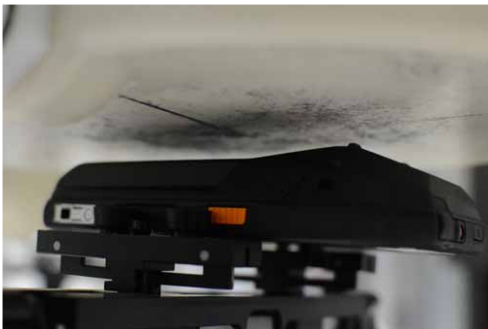
SAR Test Setup Photo 10 – Back Side at 1.0 cm with L-Battery
