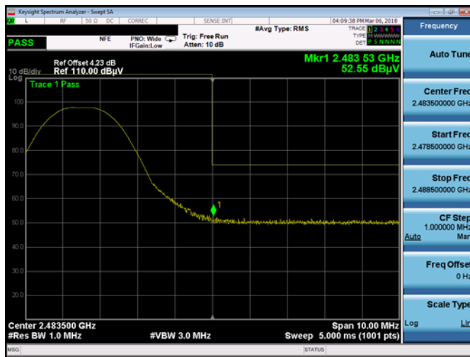
Plot 7-21. Radiated Restricted Upper Band Edge Measurement with Rugged USB Dock (Peak)
