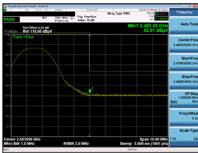
Plot 7-19. Radiated Restricted Upper Band Edge Measurement (Peak)
