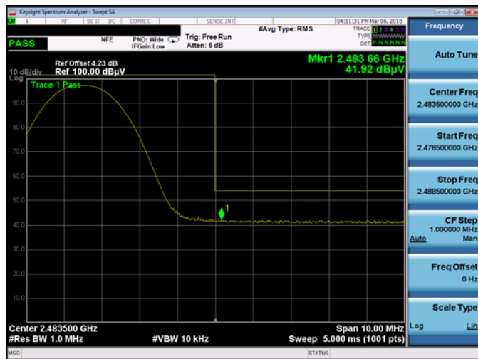
Plot 7-20. Radiated Restricted Upper Band Edge Measurement with Rugged USB Dock (Average)
