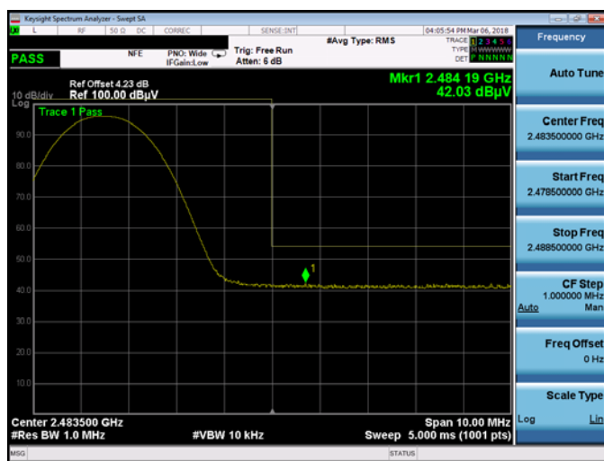
Plot 7-18. Radiated Restricted Upper Band Edge Measurement (Average)
