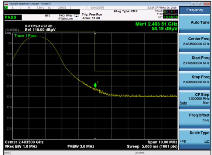
Plot 7-49. Radiated Restricted Upper Band Edge Measurement with Rugged USB Dock (Peak)
