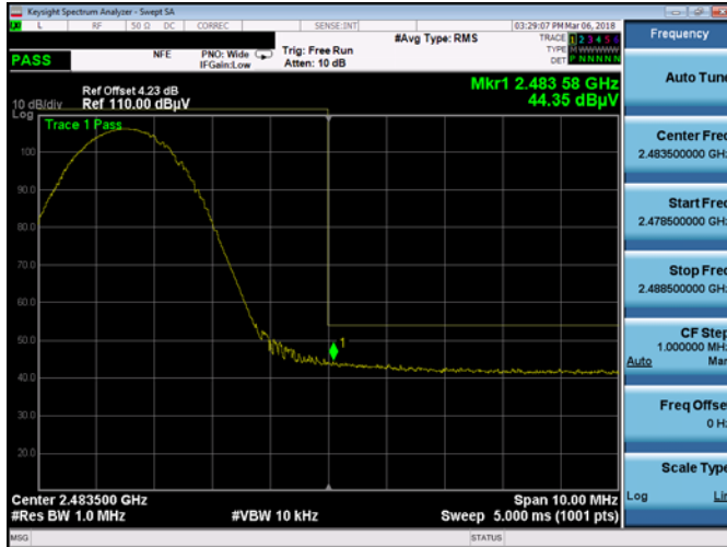
Plot 7-48. Radiated Restricted Upper Band Edge Measurement with Rugged USB Dock (Average)
