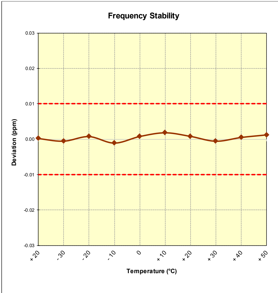
Figure 7-3. Frequency Stability Plot
