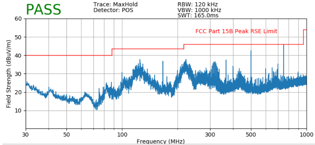
Plot 7-3. Radiated Prescan Plot (H) with Rugged USB Dock
