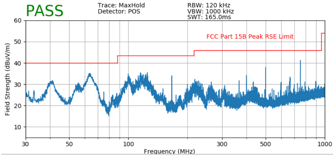
Plot 7-2. Radiated Prescan Plot (V)
