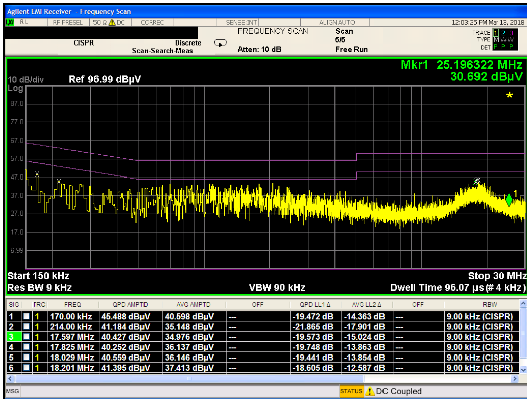
Plot 7-5. Line Conducted Plot and Data with USB(L1)
