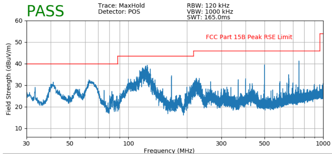
Plot 7-4. Radiated Prescan Plot (V) with Rugged USB Dock
