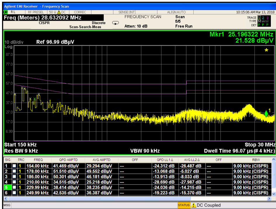
Plot 7-42. Line Conducted Plot and Data with 802.11b (L1)
