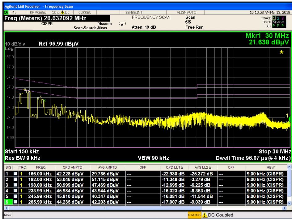
Plot 7-43. Line Conducted Plot and Data with 802.11b (N)
