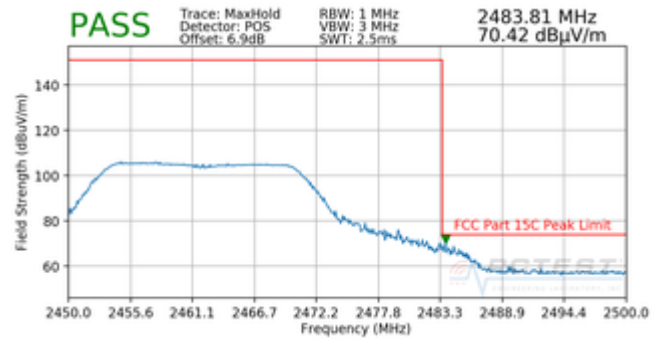
Plot 7-40. Radiated Restricted Band Edge Measurement with Rugged USB Dock (Peak)
