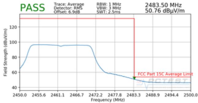
Plot 7-39. Radiated Restricted Band Edge Measurement with Rugged USB Dock (Average)
