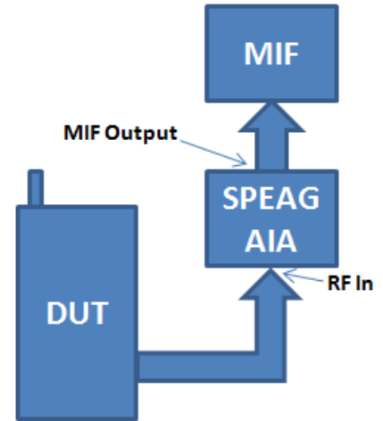
Figure 5-2 MIF Measurement Setup for unlicensed modes
