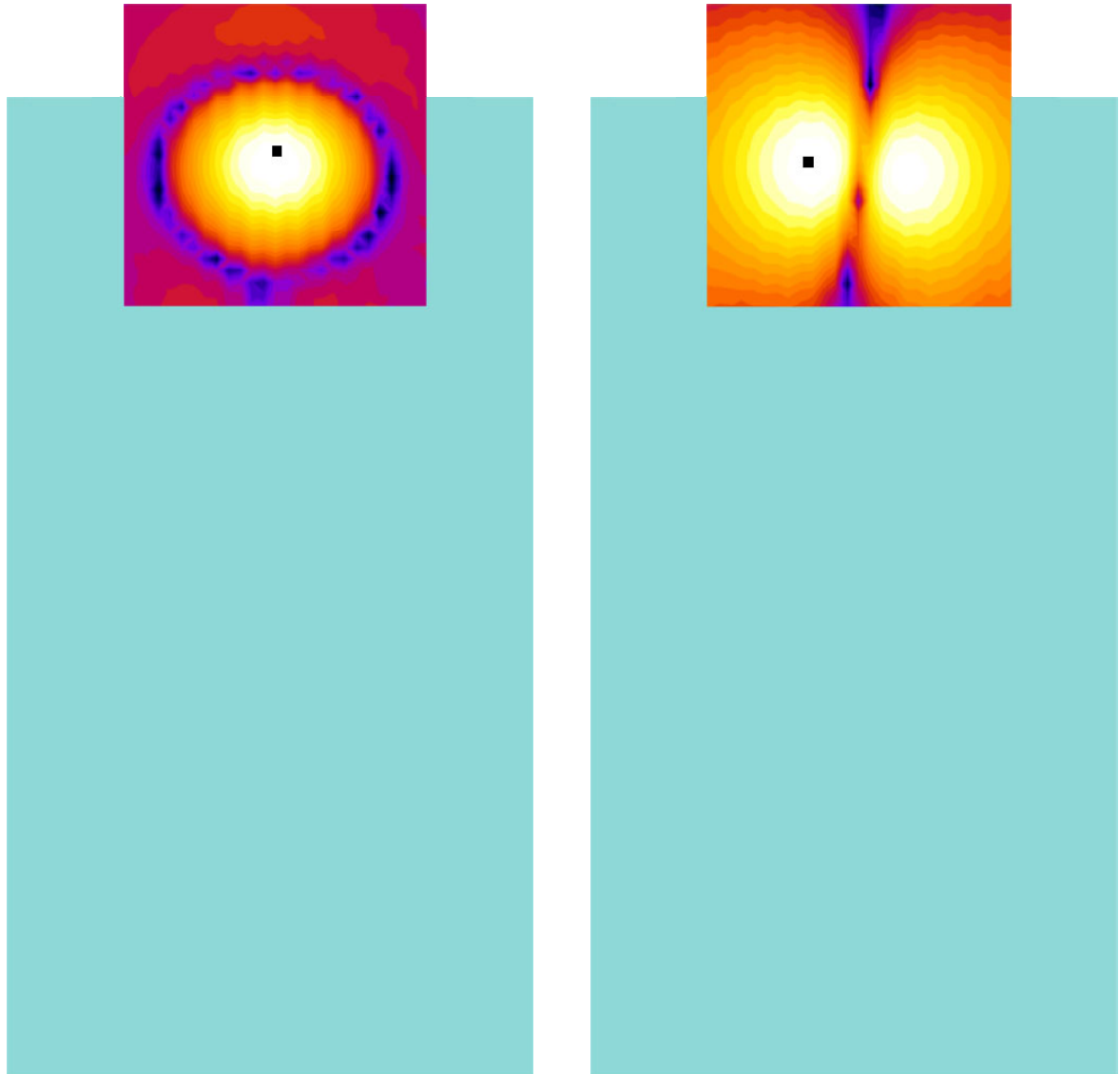
Figure 8-1 T-Coil Scan Overlay Magnetic Field Distributions
