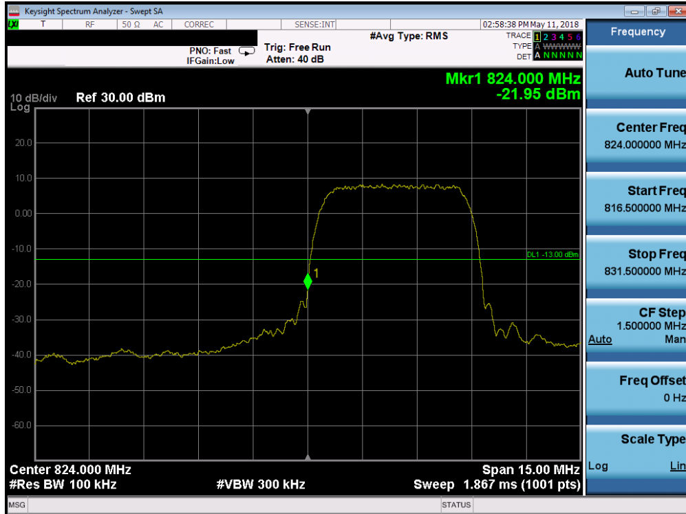
Plot 7-21. Band Edge Plot (Cellular WCDMA Mode - Low Channel)
