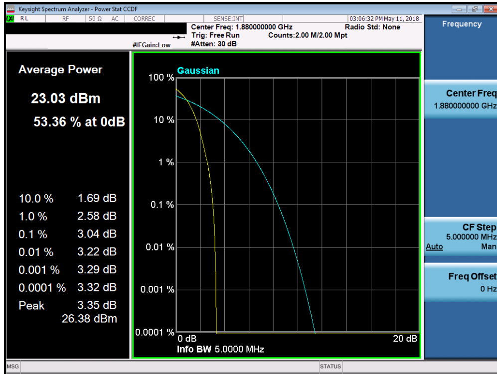
Plot 7-27. Peak-Average Ratio Plot (PCS WCDMA Mode)
