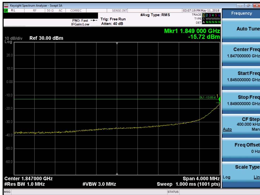
Plot 7-24. 4MHz Span Plot (PCS WCDMA Mode - Low Channel)
