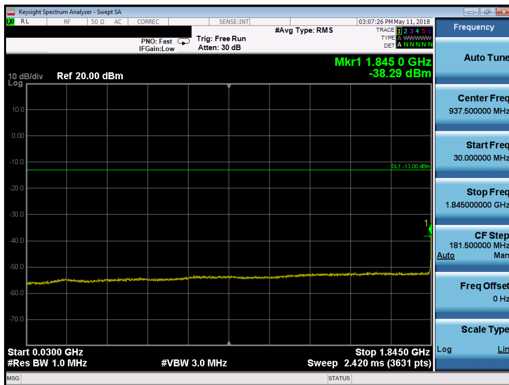
Plot 7-12. Conducted Spurious Plot (PCS WCDMA Mode - Low Channel)
