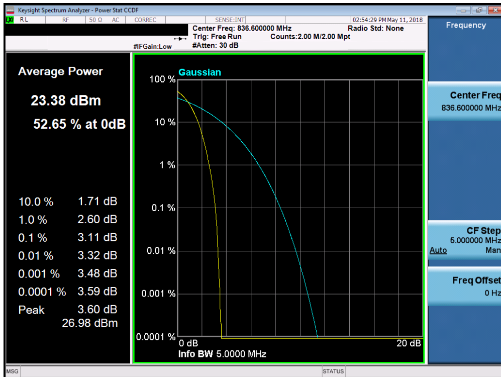
Plot 7-28. Peak-Average Ratio Plot (Cell WCDMA Mode)
