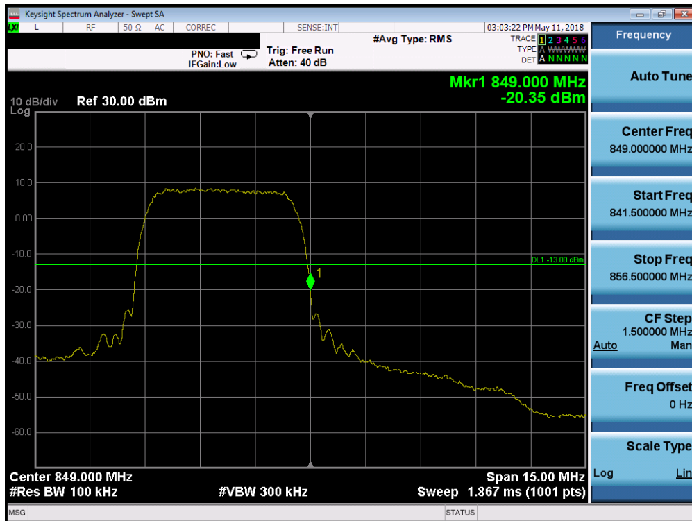
Plot 7-22. Band Edge Plot (Cellular WCDMA Mode - High Channel)
