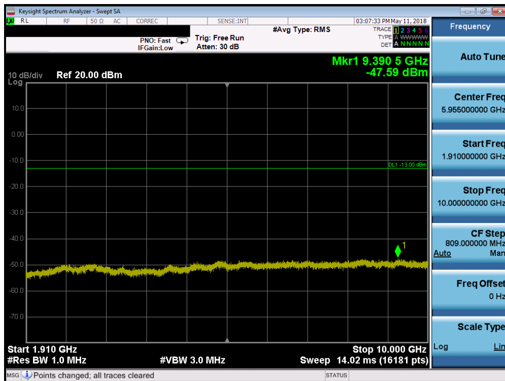
Plot 7-13. Conducted Spurious Plot (PCS WCDMA Mode - Low Channel)
