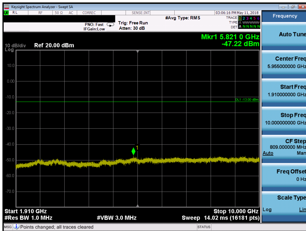
Plot 7-16. Conducted Spurious Plot (PCS WCDMA Mode - Mid Channel)
