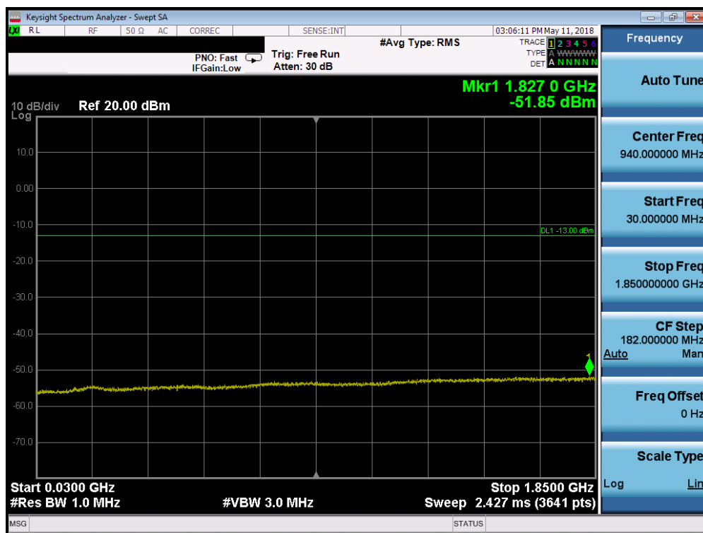
Plot 7-15. Conducted Spurious Plot (PCS WCDMA Mode - Mid Channel)
