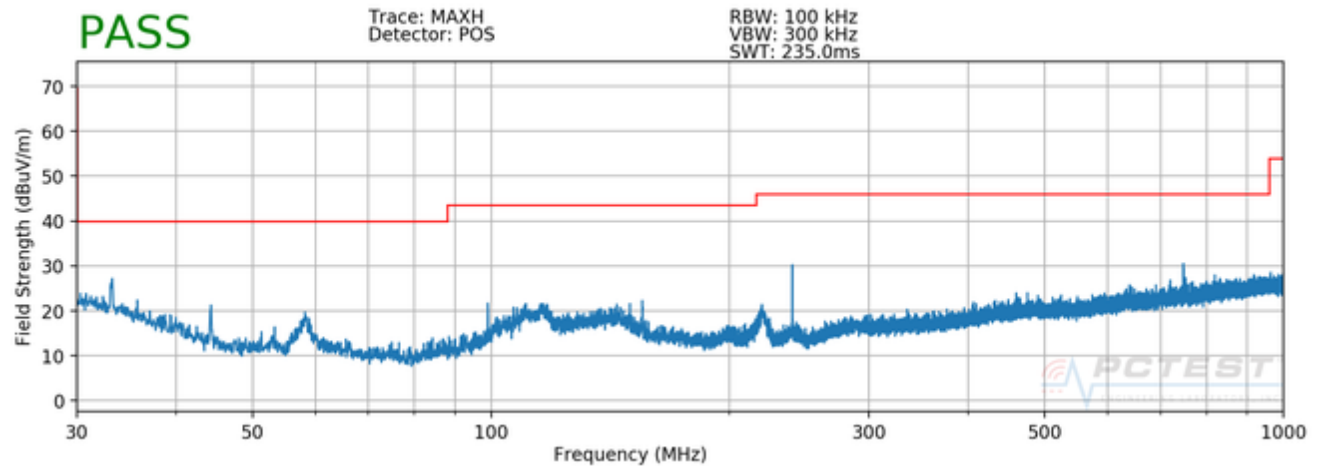
Plot 7-2. Radiated Prescan Plot (V)
