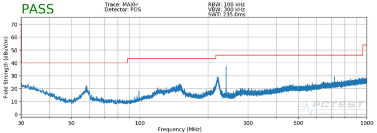
Plot 7-1. Radiated Prescan Plot (H)
