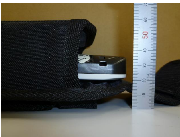
When the device attached the holster is away human body 20mm.
