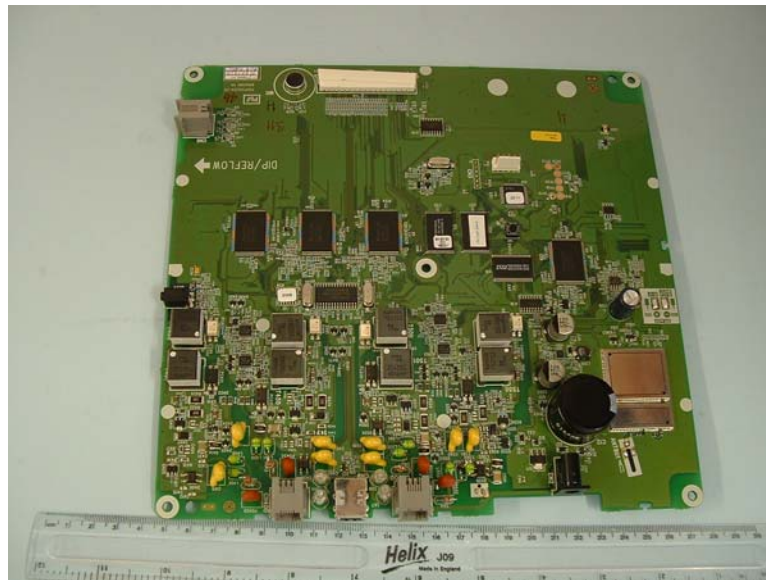
MAIN PCB COMPONENT SIDE
