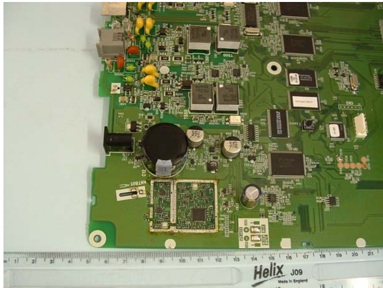
PHOTOGRAPH No. 7 MAIN PCB COMPONENT SIDE CAN REMOVED
