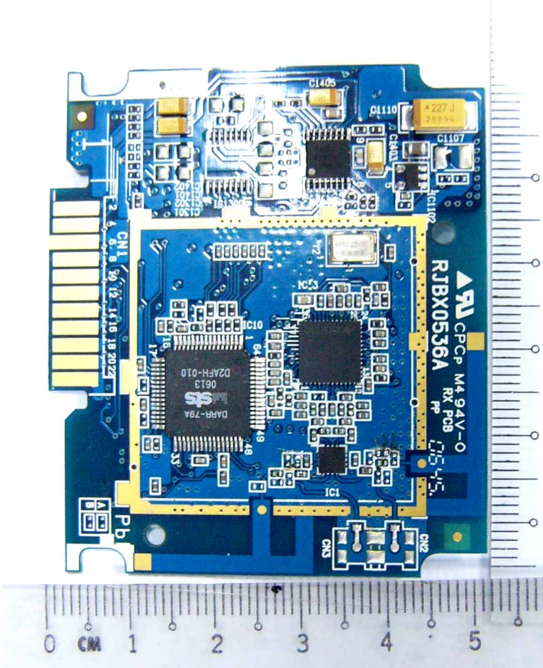
Receiver ( Front View ) RF Shield Removed
