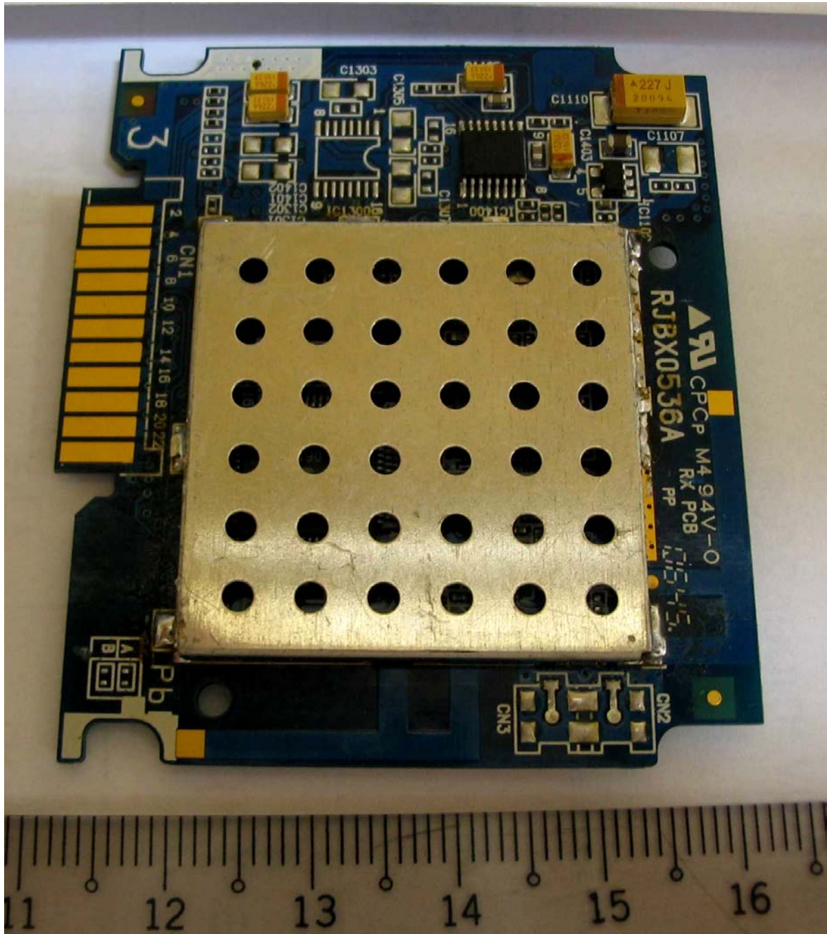
Receiver ( Front View )
