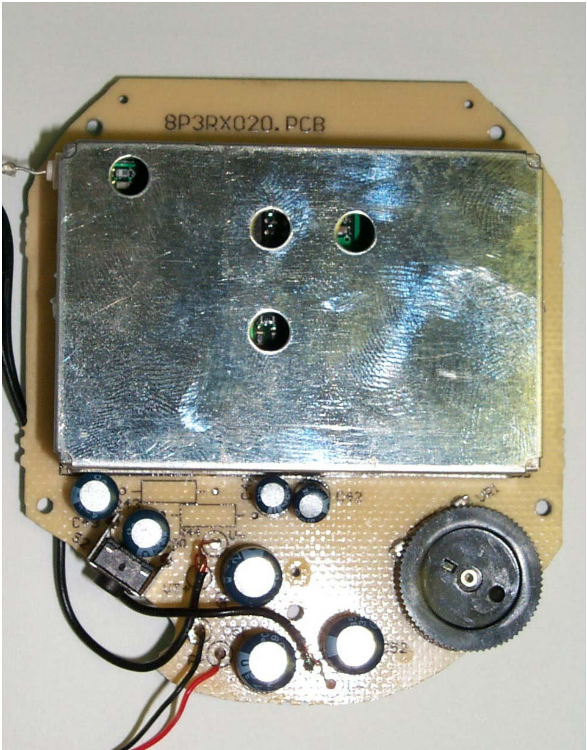
Figure 7.5 Right Side PBC Component Side
