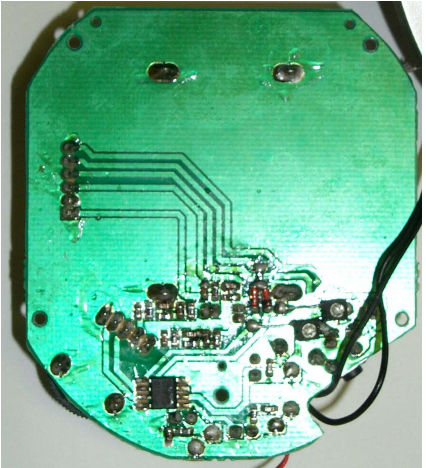
Figure 7.6 Right Side PBC Foil Side
