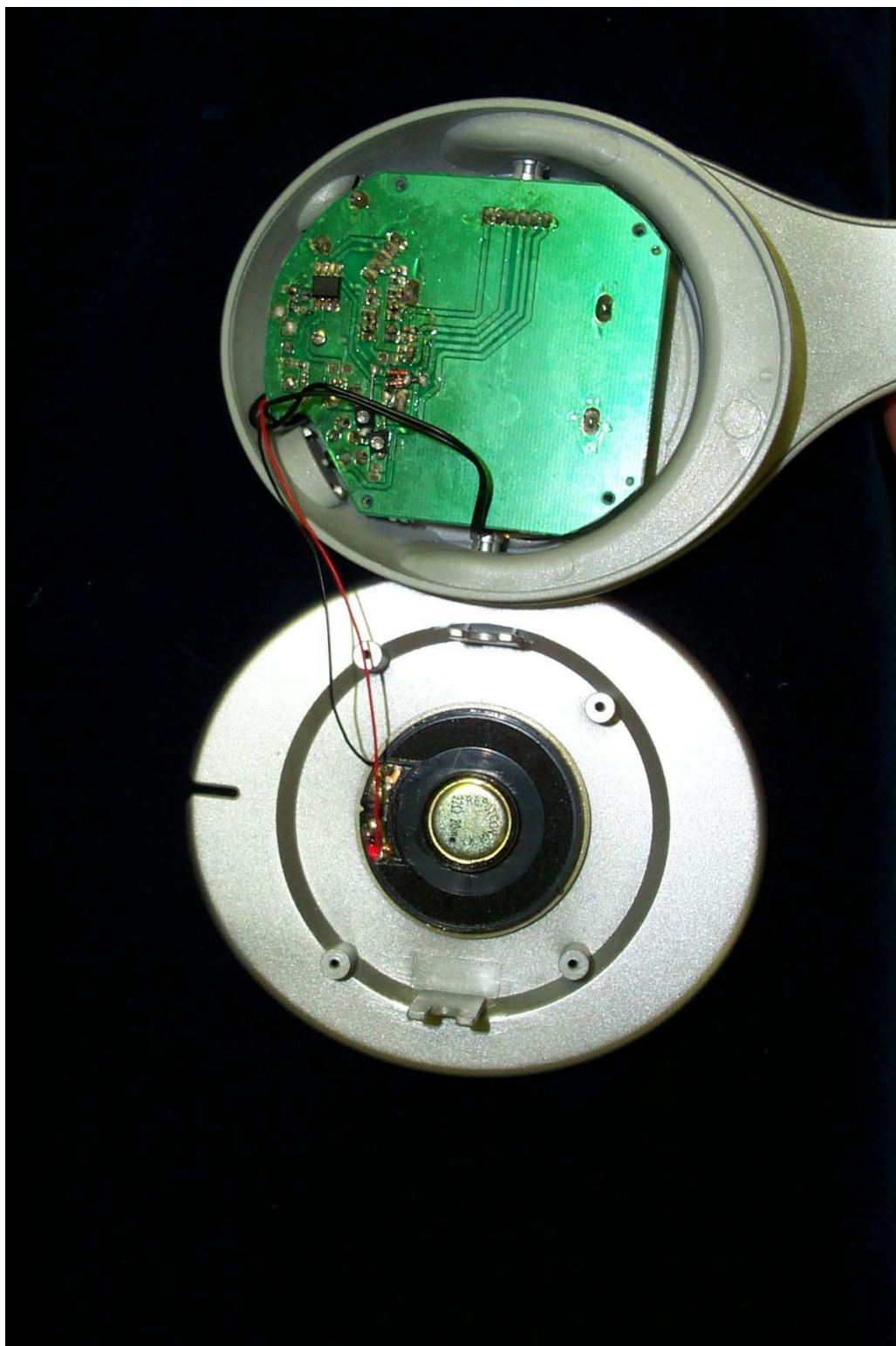
Figure 7.4 Right Side Open View
