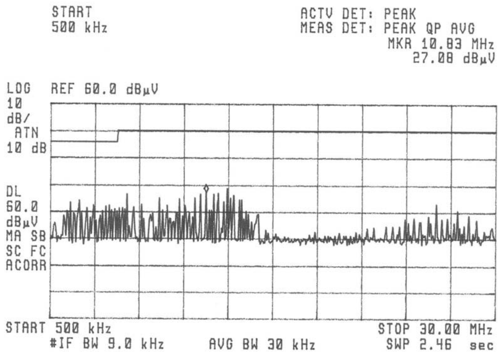
Figure 5.1 Line Conducted
