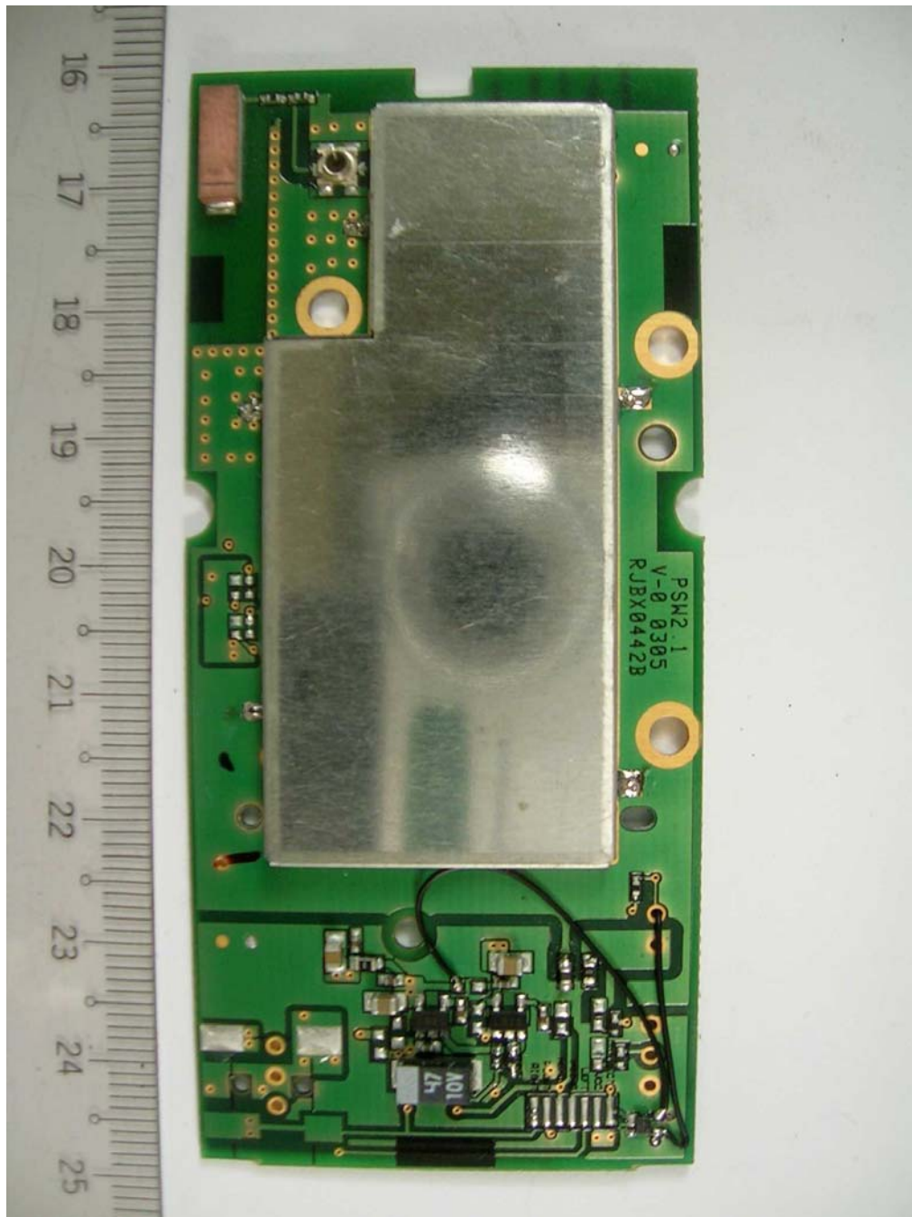
EUT PCB Top View (With RF Shield)
