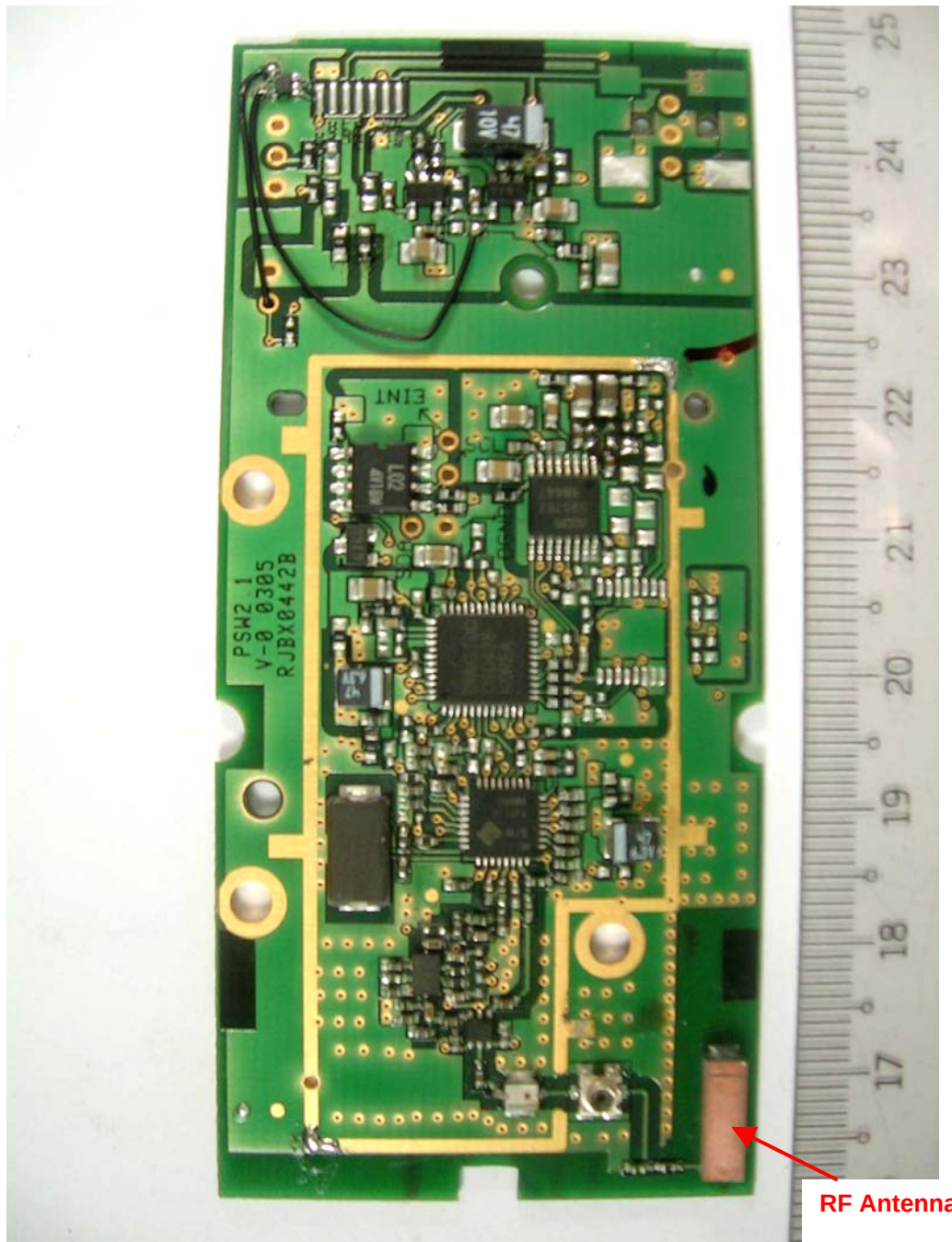
EUT PCB Top View (With RF Shield Removed)
