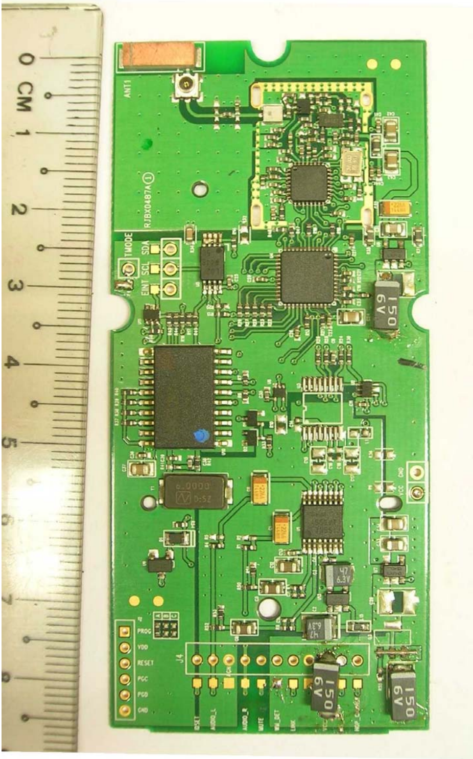
Front View (RF Shield Removed)
