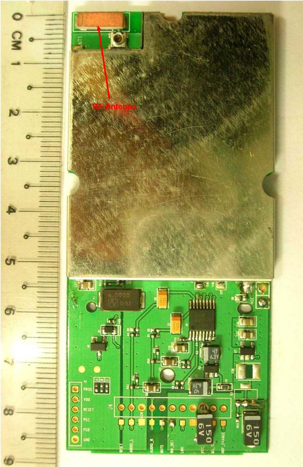
Front View (with RF Shield)
