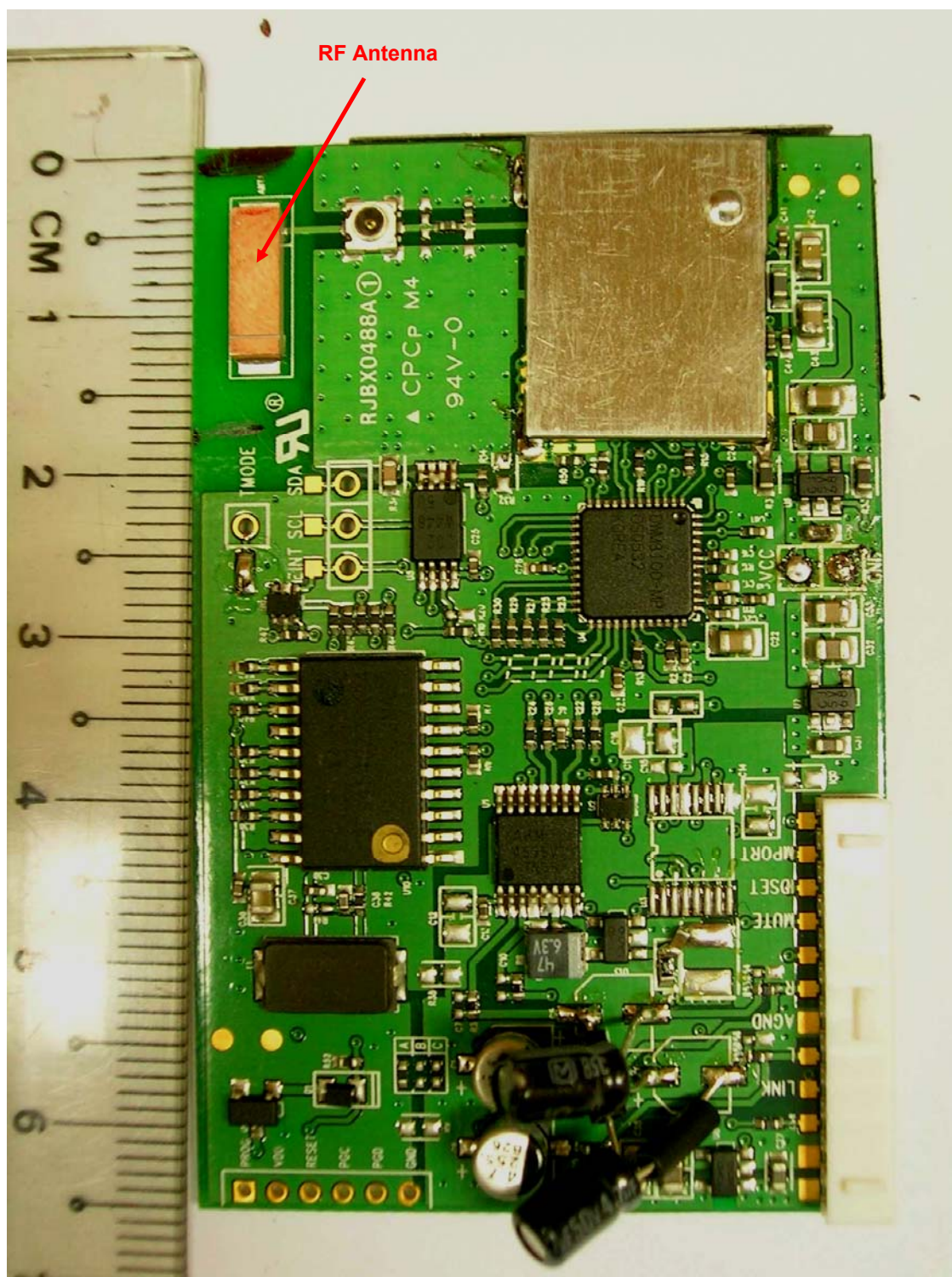
Front View (with RF Shield)
