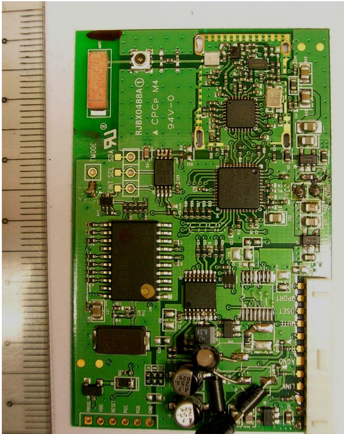
Front View (RF Shield Removed)
