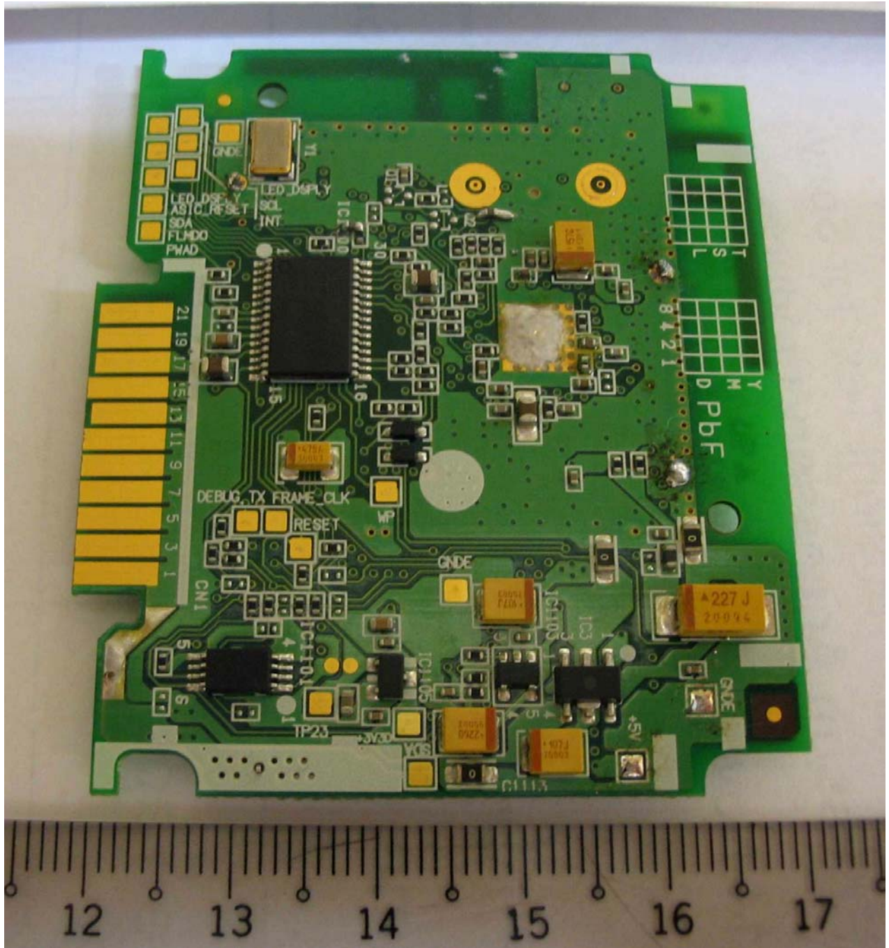
Transmitter ( Rear View ) RF Shield Removed
