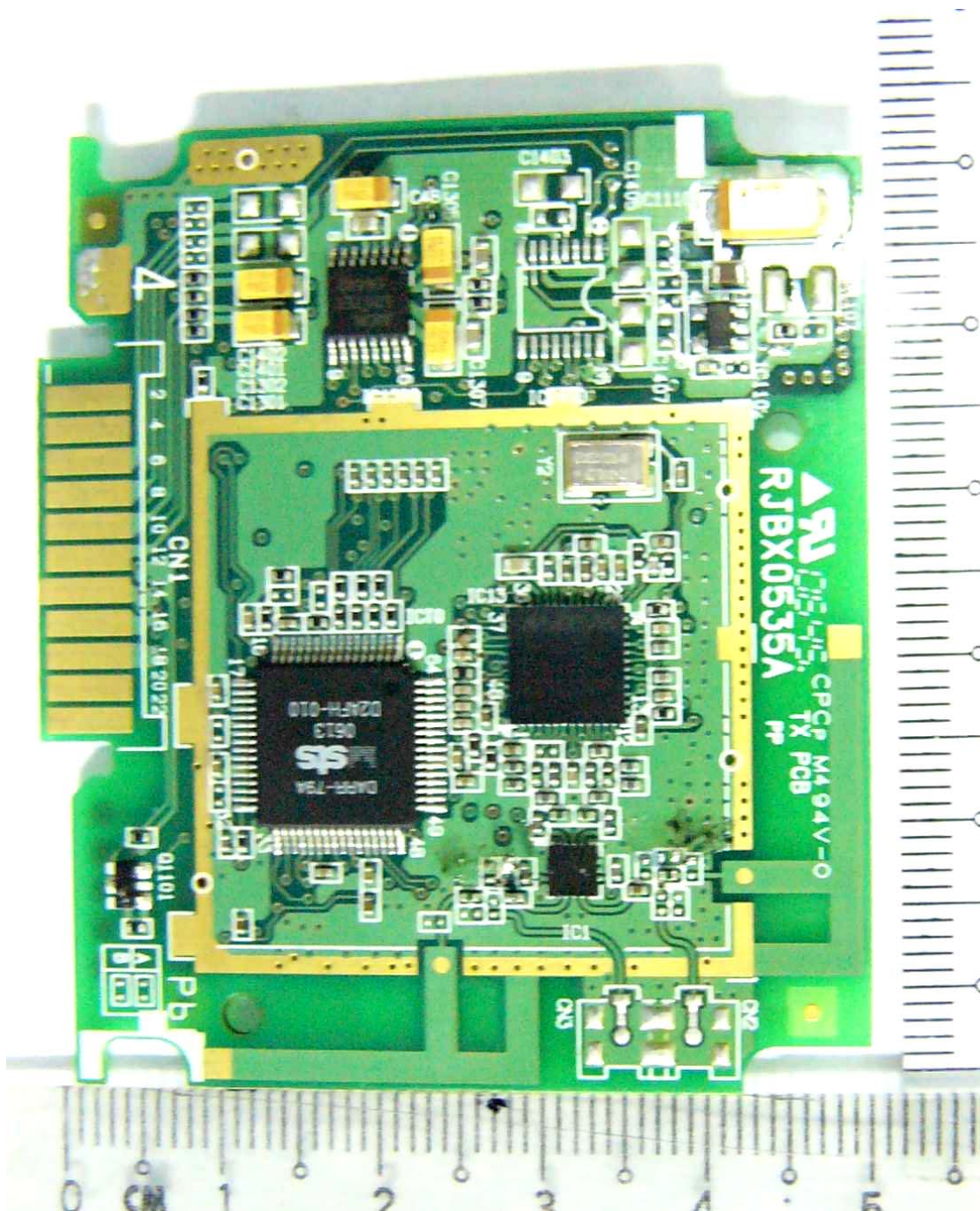
Transmitter ( Front View ) RF Shield Removed
