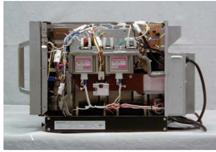
Exhibit 2-D2 Right Side View NE-C1173 No Enclosure
