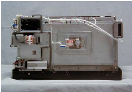
Exhibit 2-E2 Rear View NE-C1173 No Enclosure
