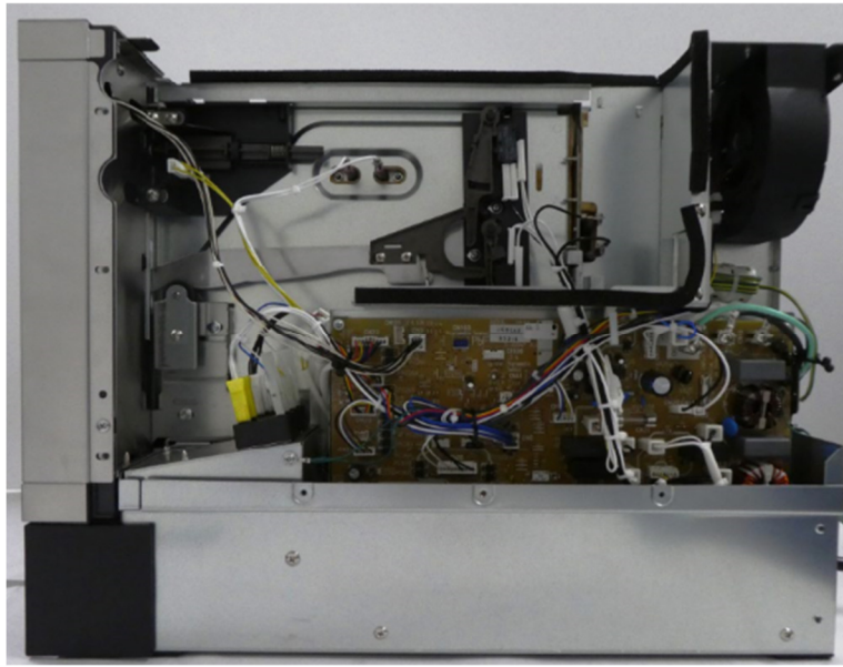
Rear View without Enclosure
