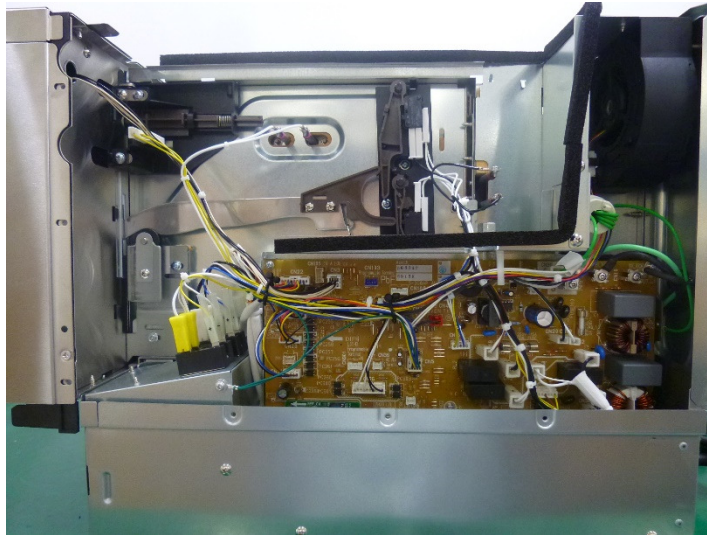
Right Side View without Enclosure
