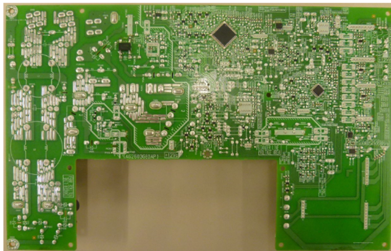
Top and Bottom View of Power Relay Board
