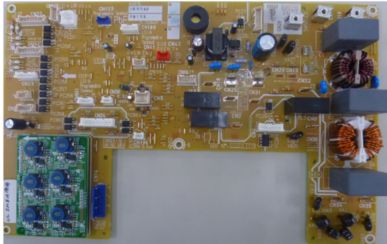
Top and Bottom View of Power Supply Board
