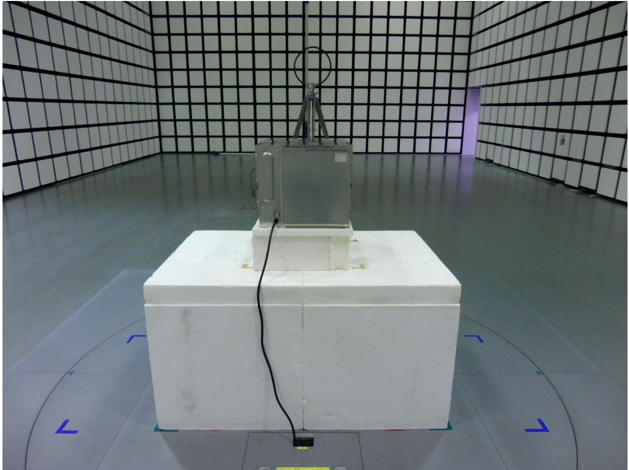
EXHIBIT D – TEST SETUP PHOTOS (9kHz to 30MHz)
