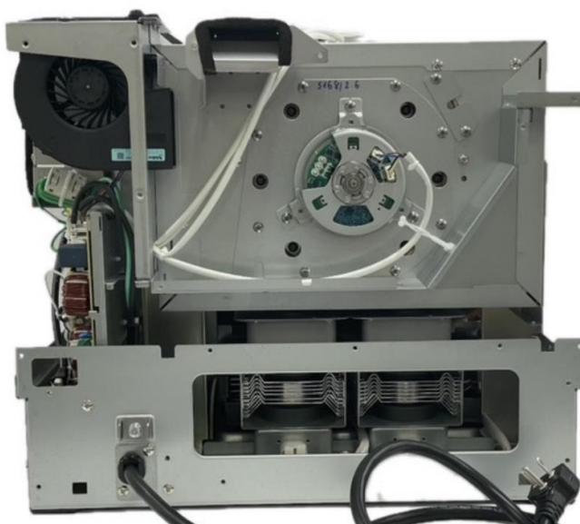
Rear View without Enclosure
