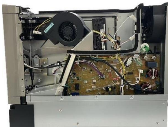
Left Side View without Enclosure
