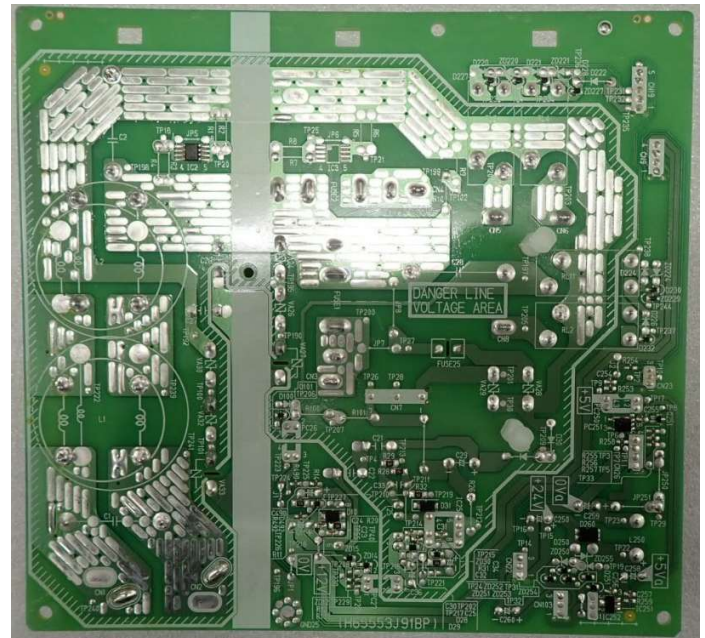
Top and bottom view of PCB D UNIT (Power supply, Power relay, Line noise filter Board)
