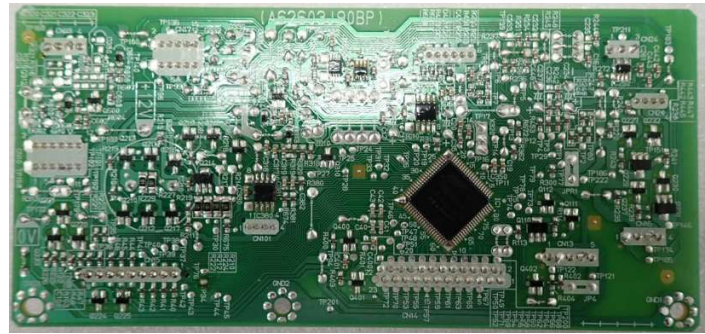
Top and bottom view of PCB D UNIT (Power supply, Power relay, Line noise filter Board)
