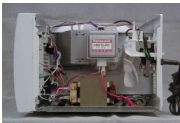
Exhibit 2-D2 Right side view, no enclosure NN-MX25WF
