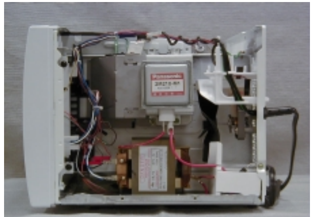
Exhibit 2-D2 Right side view, No enclosure NN-GX35WF
