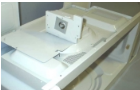
Exhibit 2-H2; View of Magnetron Waveguide
