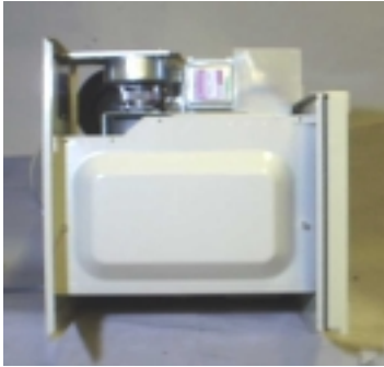
Exhibit 2-C2; Left Side View no enclosure, NN-S262WF
