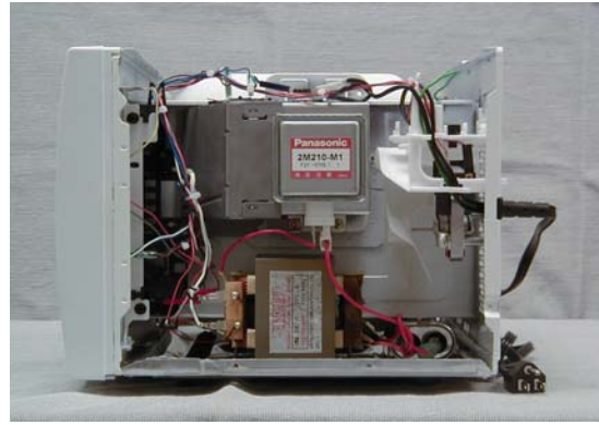
Exhibit 2-D2 Right side view, No enclosure NN-MX26 BF
