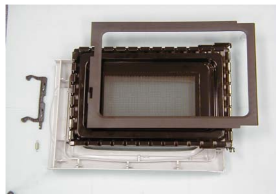
Exhibit 2-I View of Door Choke Constructi
