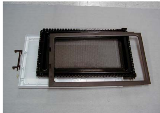
Exhibit 2-I View of Door Choke Construction
