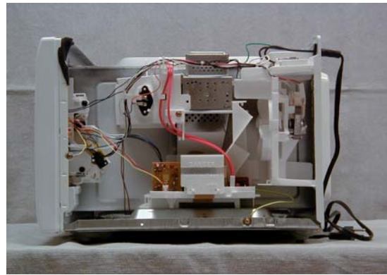
Exhibit 2-D2 Right side view, No enclosure NN-S963WF
