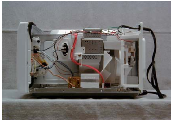
Exhibit 2-D2 Right side view, No enclosure NN-S763WF
