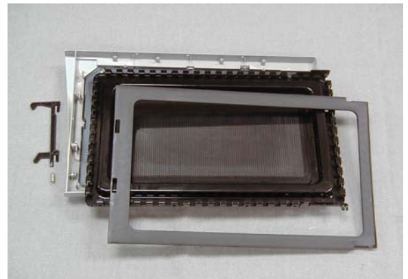
Exhibit 2-I View of Door Choke Constructio
