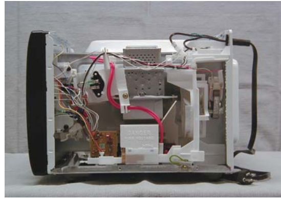
Exhibit 2-D2 Right side view, No enclosure NN-S563BF
