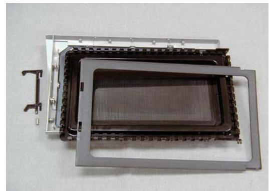
Exhibit 2-I View of Door Choke (C)
