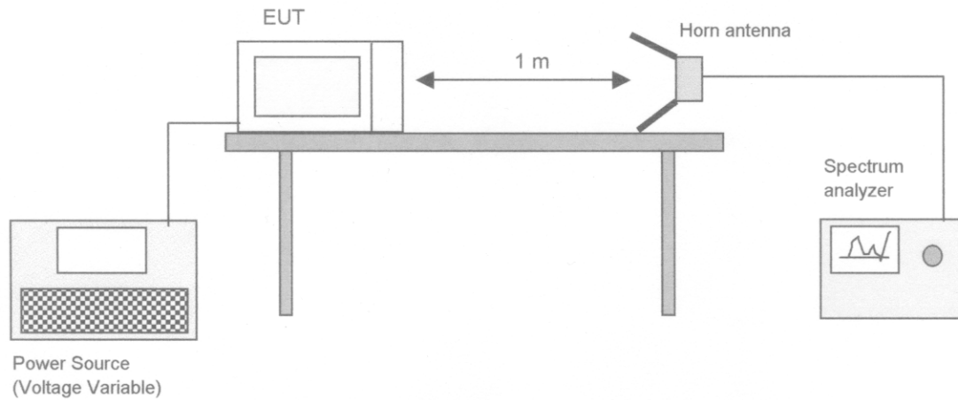
Fig. 4 Operating Frequency Measurements Configuration
