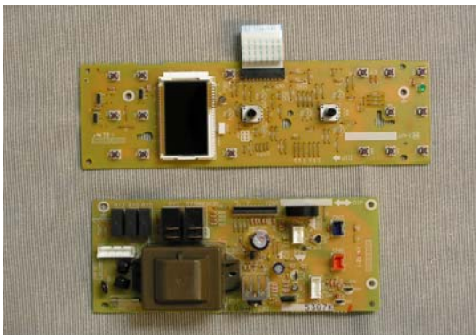
Exhibit 2-I View of Control Circuitry
