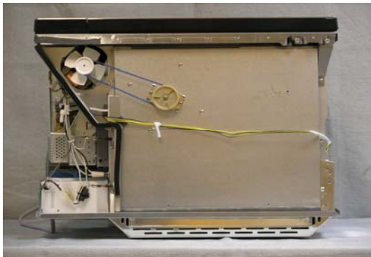
Exhibit 2-F2 Top view, No enclosure NN-C994SF
