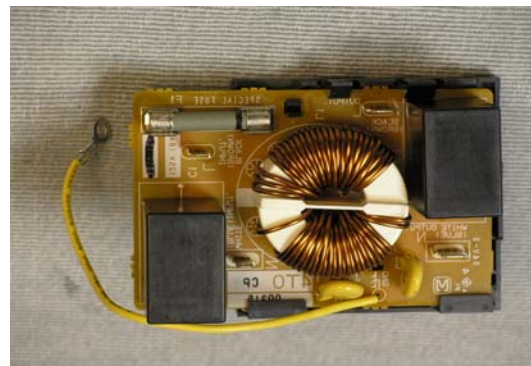
Exhibit 2-J View of Power Line Filter Circuitry
