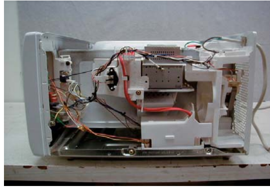
Exhibit 2-D2 Right side view, No enclosure NN-S754WF
