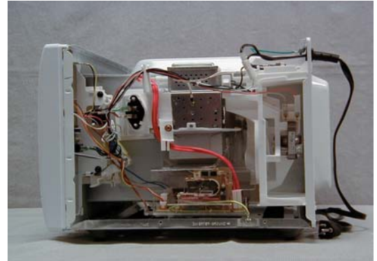
Exhibit 2-D2 Right side view, No enclosure NN-S654BF
