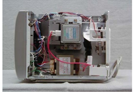
Exhibit 2-D2 Right Side View No Enclosure NN-G355
