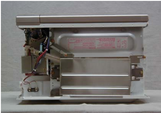
Exhibit 2-F2 Top View No Enclosure NN-G355MF
