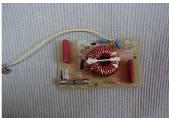
Exhibit 2-G2 Bottom view, No enclosure NN-P295SF
