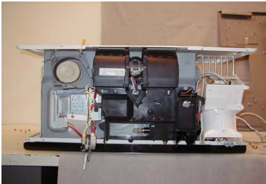
Exhibit 2-F2 Top view, No enclosure NN-P295SF
