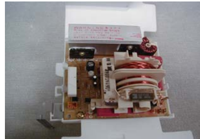
Exhibit 2-J View of Inverter Circuitry
