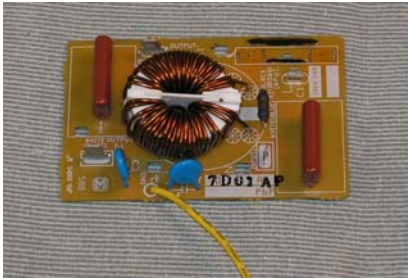
Exhibit 2-L1 View of Power Line Filter Circuitry (New Submission) (Alternate Construction)
