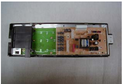
Exhibit 2-H View of Control Circuitry
