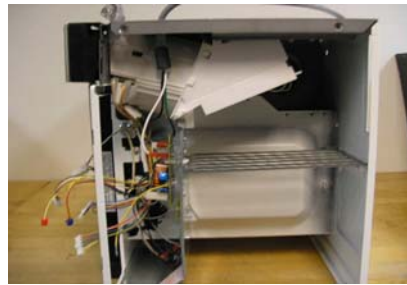
Exhibit 2-D1A Right side view, No enclosure NN-P295SF (New Submission) (Alternate Construction)
