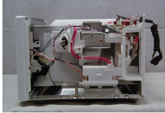
Exhibit 2-D2 Right side view, No enclosure NN-H965WF
