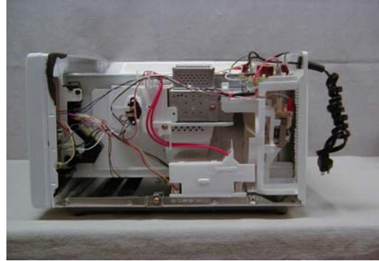
Exhibit 2-D2 Right side view, No enclosure NN-H765WF
