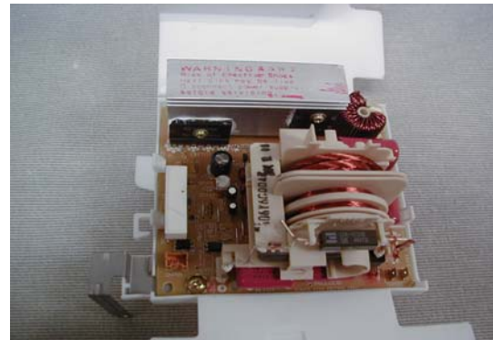
Exhibit 2-J View of Inverter Circuitry
