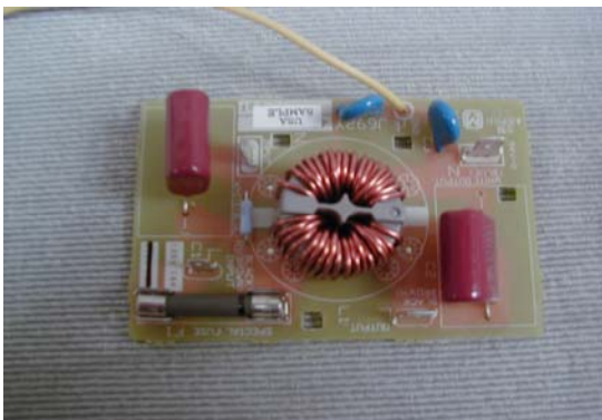
Exhibit 2-I View of Power Line Filter Circuitry
