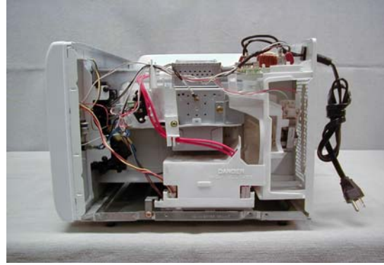
Exhibit 2-D2 Right side view, No enclosure NN-H665WF
